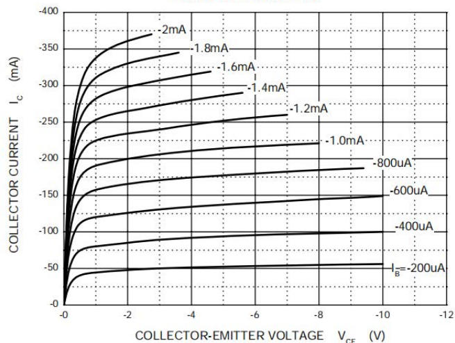
Static Characteristic
