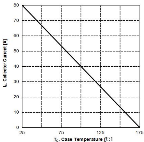
Figure 2: Collector Current vs. Case Temperature
