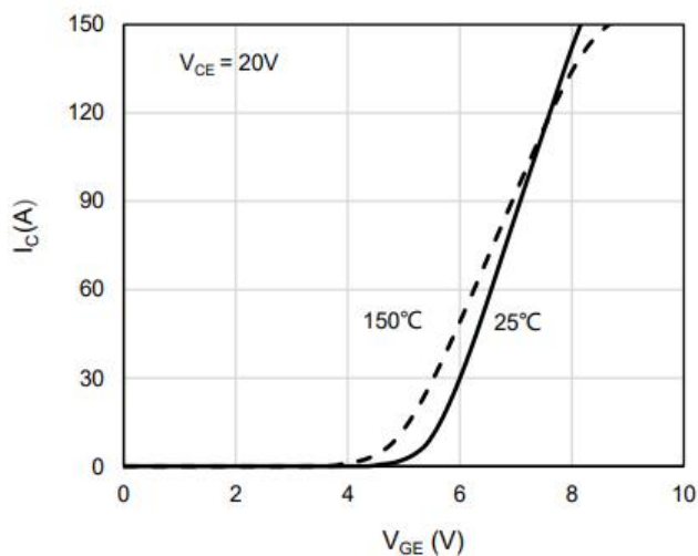
Fig.6 Transfer characteristics
