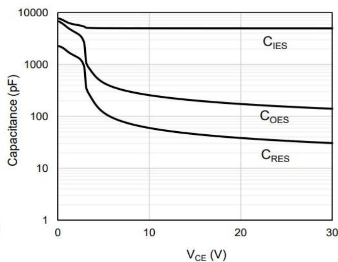
Fig.6 Typical capacitance
