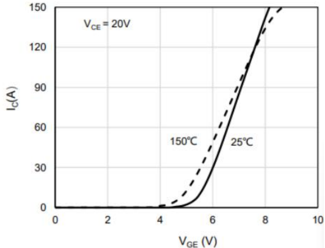
Fig.4 Transfer characteristics
