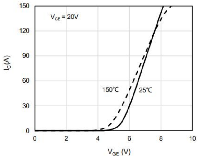
Fig.6 Transfer characteristics
