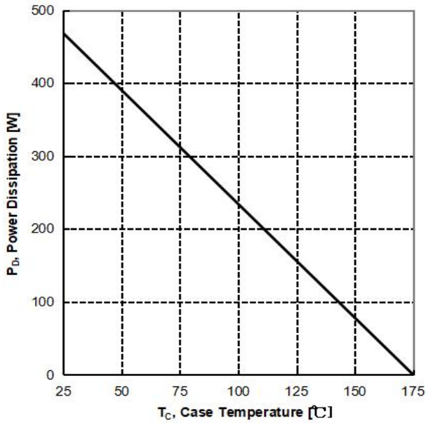
Figure 1: Power Dissipation
