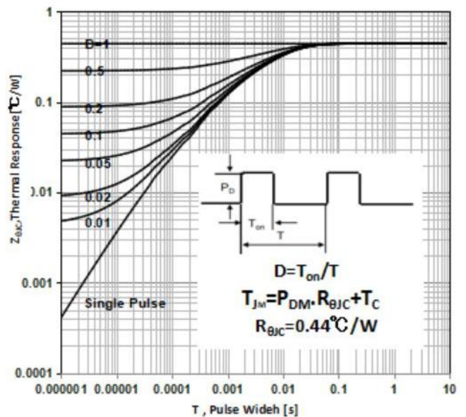
Figure 20: Diode Transient Thermal Impedance vs. Pulse Width
