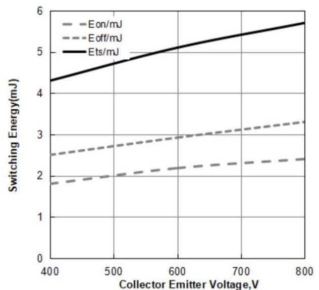
Figure 16: Typical Switching Energy vs. V_{CE} ( T_J=25^{\circ}\text{C} , V_{GE}=15\text{V} , I_C=60\text{A} , R_g=5\Omega )
