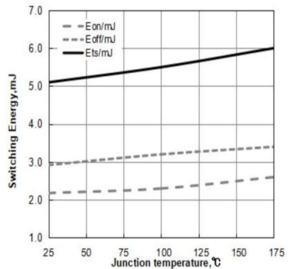
Figure 12: Typical Switching Energy vs. Junction Temperature ( V_{CE}=600\text{V} , V_{GE}=15\text{V} , I_C=60\text{A} , R_g=5\Omega )
