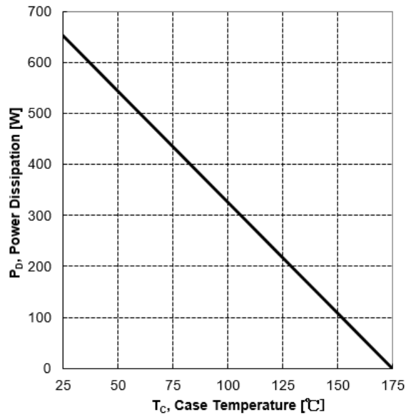
Figure 1: Power Dissipation
