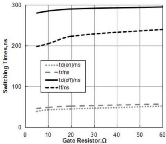
Figure 9: Typical Switching Times vs. Gate Resistor ( T_J=25^{\circ}\text{C} , V_{CE}=600\text{V} , V_{GE}=15\text{V} , I_C=60\text{A} )
