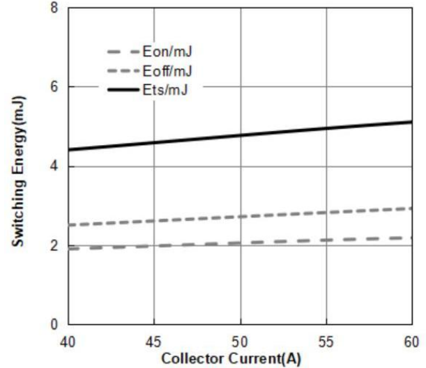
Figure 14: Typical Switching Energy vs. Collector Current ( T_J=25^{\circ}\text{C} , V_{CE}=600\text{V} , V_{GE}=15\text{V} , R_g=5\Omega )
