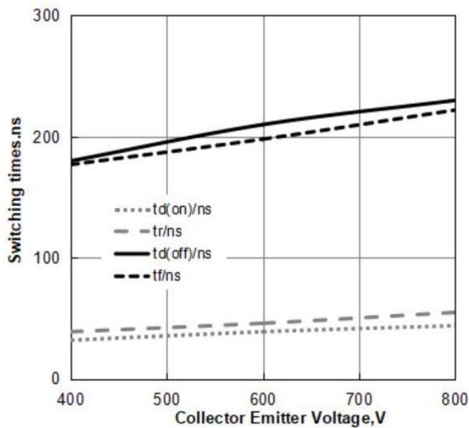
Figure 15: Typical Switching Times vs. V_{CE} ( T_J=25^{\circ}\text{C} , V_{GE}=15\text{V} , I_C=60\text{A} , R_g=5\Omega )
