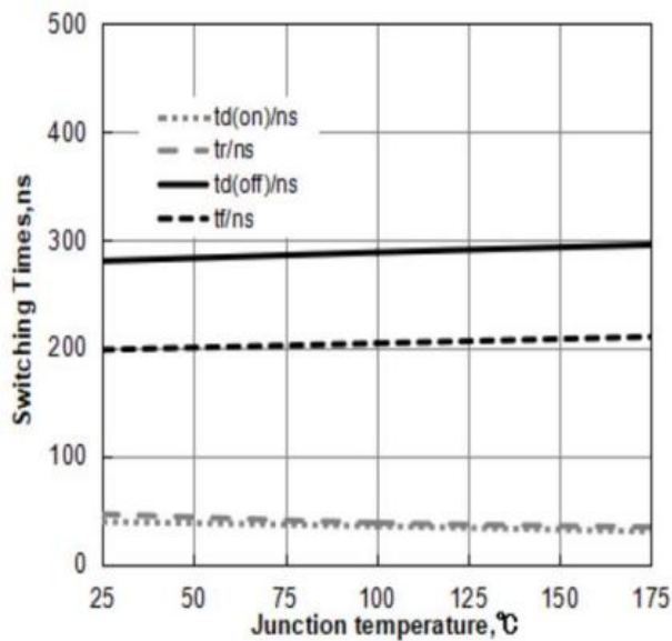
Figure 11: Typical Switching Times vs. Junction Temperature ( V_{CE}=600\text{V} , V_{GE}=15\text{V} , I_C=60\text{A} , R_g=5\Omega )
