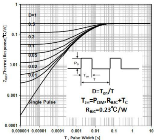
Figure 19: IGBT Transient Thermal Impedance vs. Pulse Width
