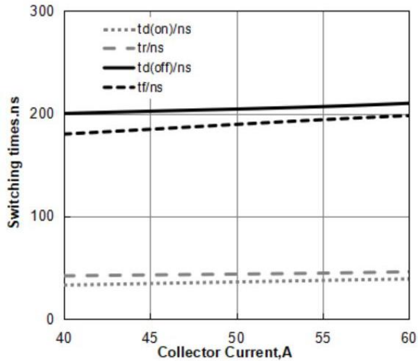
Figure 13: Typical Switching Times vs. Collector Current ( T_J=25^{\circ}\text{C} , V_{CE}=600\text{V} , V_{GE}=15\text{V} , R_g=5\Omega )
