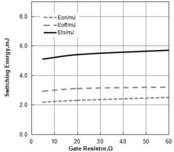
Figure 10: Typical Switching Energy vs. Gate Resistor ( T_J=25^{\circ}\text{C} , V_{CE}=600\text{V} , V_{GE}=15\text{V} , I_C=60\text{A} )
