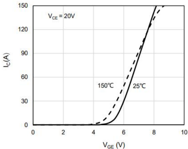
Fig.6 Transfer characteristics
