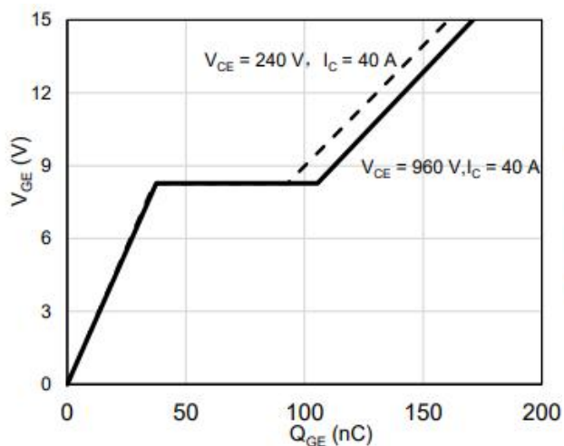
Fig.5 Gate charge
