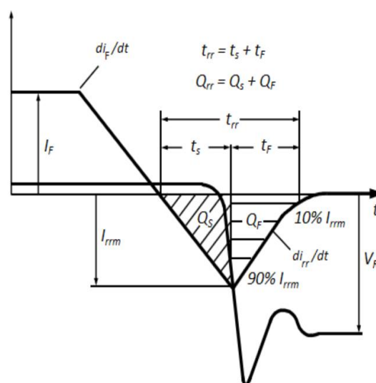
Figure 25. Definition of diode switching characteristics
