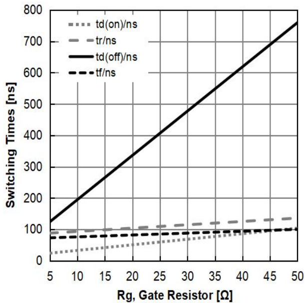
Figure 9: Typical Switching Times vs. Gate Resistor ( T_J=25^{\circ}\text{C} , V_{CE}=400\text{V} , V_{GE}=15\text{V} , I_C=60\text{A} )
