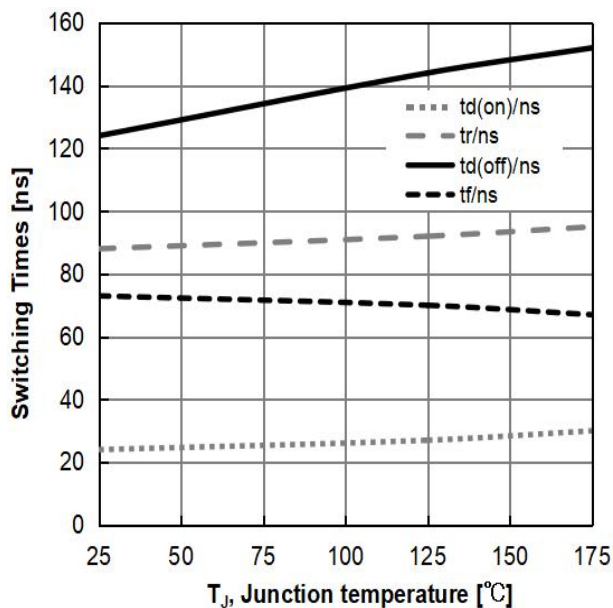
Figure 11: Typical Switching Times vs. Junction Temperature ( V_{CE}=400\text{V} , V_{GE}=15\text{V} , I_C=60\text{A} , R_g=5\Omega )
