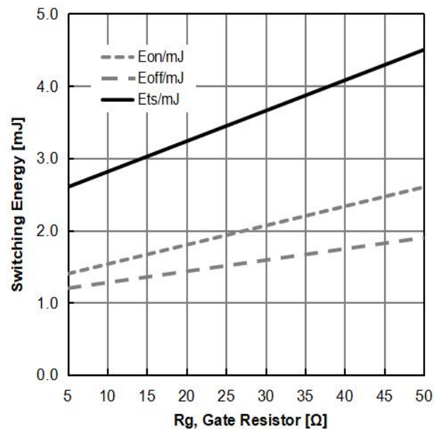
Figure 10: Typical Switching Energy vs. Gate Resistor ( T_J=25^{\circ}\text{C} , V_{CE}=400\text{V} , V_{GE}=15\text{V} , I_C=60\text{A} )
