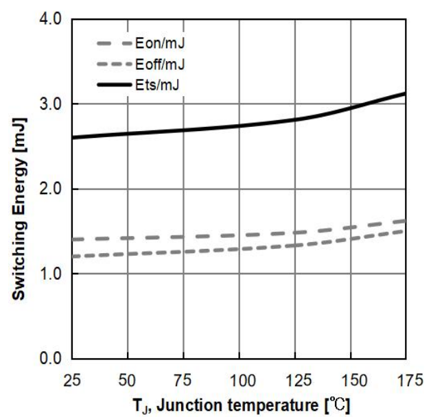
Figure 12: Typical Switching Energy vs. Junction Temperature ( V_{CE}=400\text{V} , V_{GE}=15\text{V} , I_C=60\text{A} , R_g=5\Omega )
