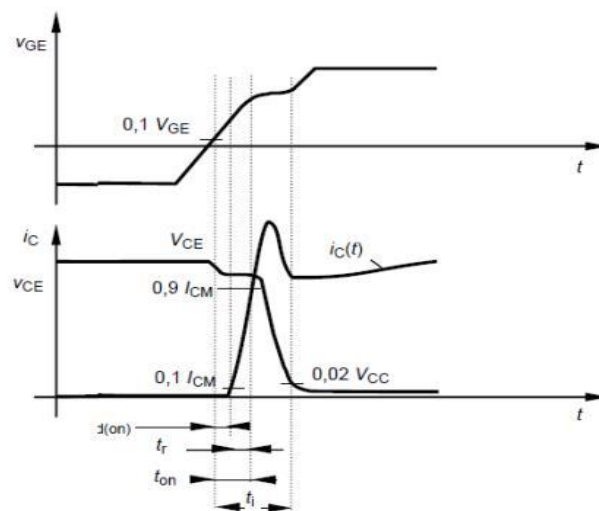
Switching Test Circuit & Waveforms
