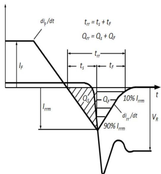
Figure 25. Definition of diode switching characteristics
