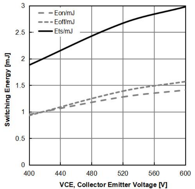
Figure 16: Typical Switching Energy vs. V_{CE} ( T_J=25^{\circ}\text{C} , V_{GE}=15\text{V} , I_C=40\text{A} , R_g=5\Omega )
