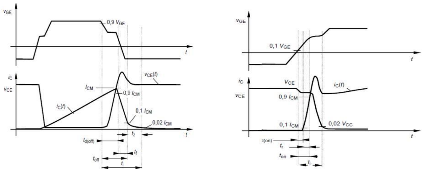
Switching Test Circuit & Waveforms
