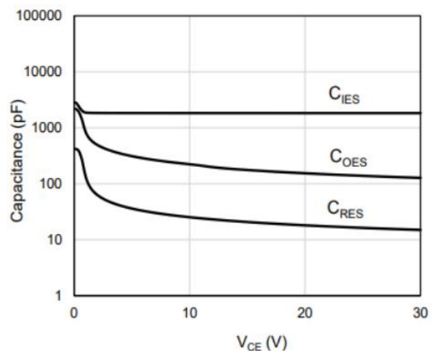
Fig.6 Typical capacitance
