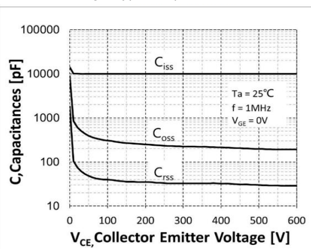
Fig.6 Typical capacitance
