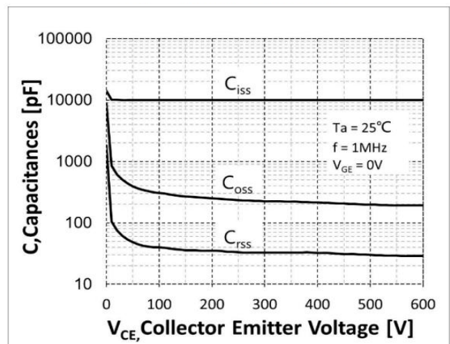
Fig.6 Typical capacitance
