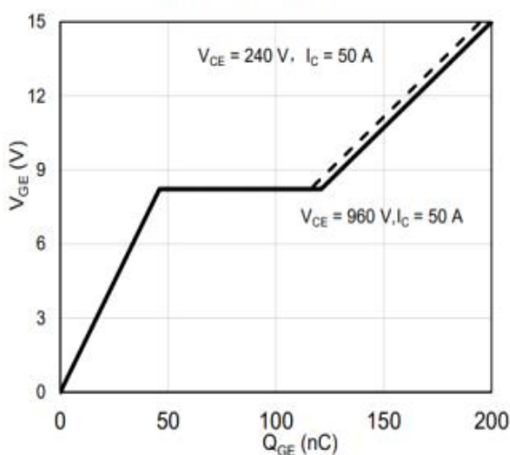
Fig.5 Gate charge
