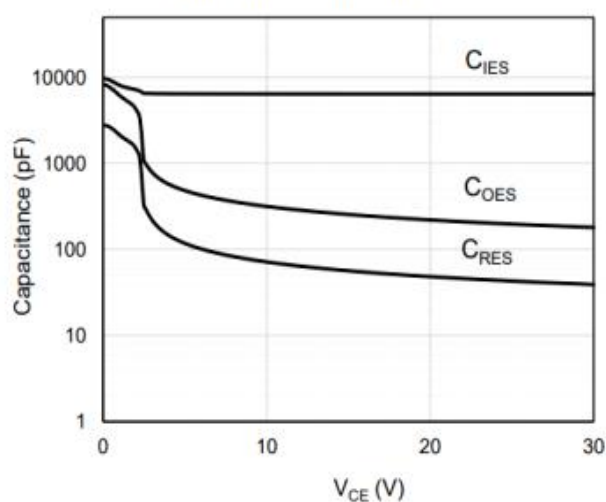
Fig.6 Typical capacitance
