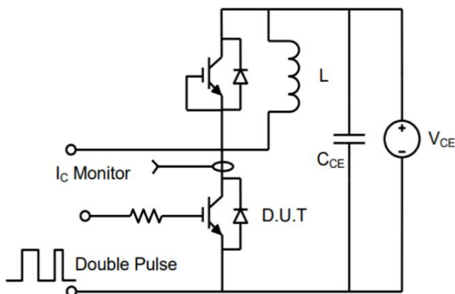
Diode Recovery Test Circuit & Waveforms
