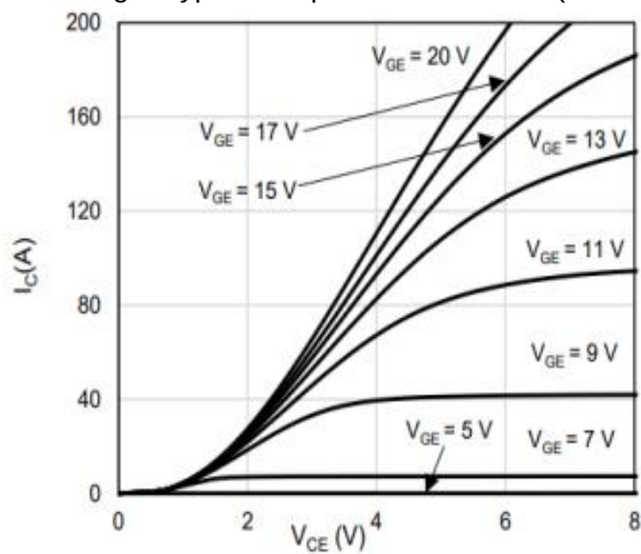
Fig.2 Typical Output characteristics (175°C)
