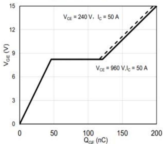
Fig.5 Gate charge
