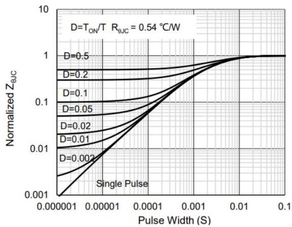
Fig.13 Transient Thermal Impedance Diode
