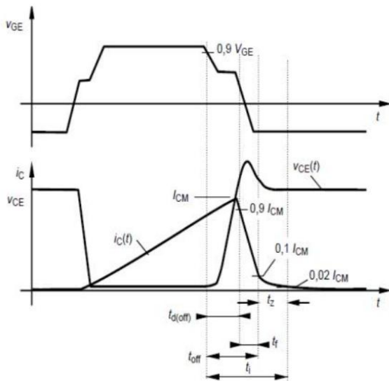
Switching Test Circuit & Waveforms
