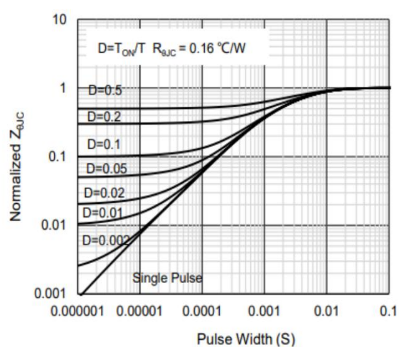
Fig.12 Transient Thermal Impedance IGBT
