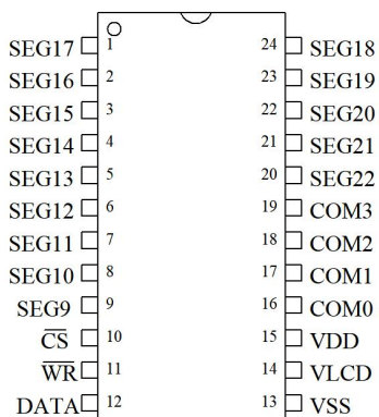
HT1621B SOP/SSOP-24
