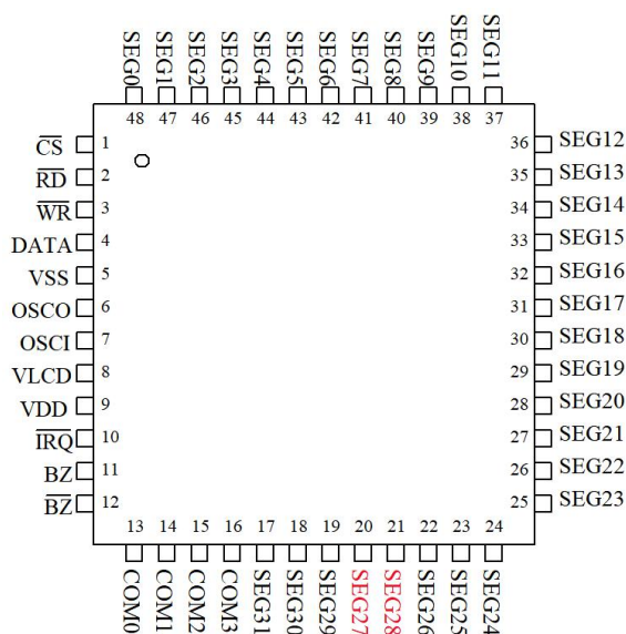
CS1621 LQFP-48
