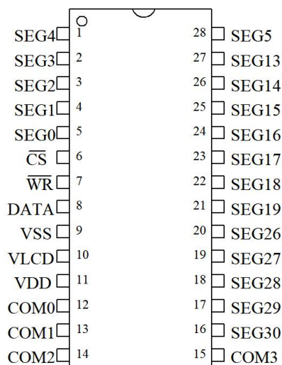
CS1621 SOP/SSOP-28
