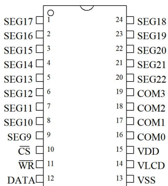
CS1621 SOP/SSOP-24
