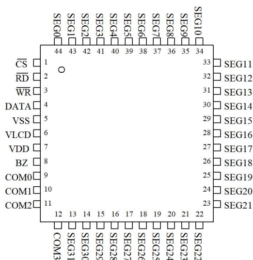
CS1621 LQFP-44
