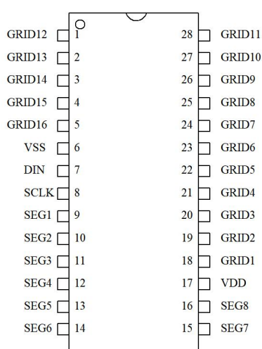
HTM1640 SOP/SSOP-28
