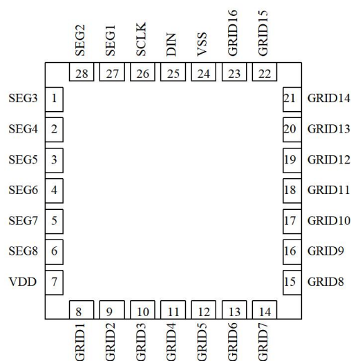
HTM1640 QFN4X4-28L
