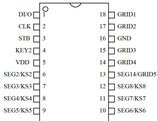
HTM1630 DIP-18
