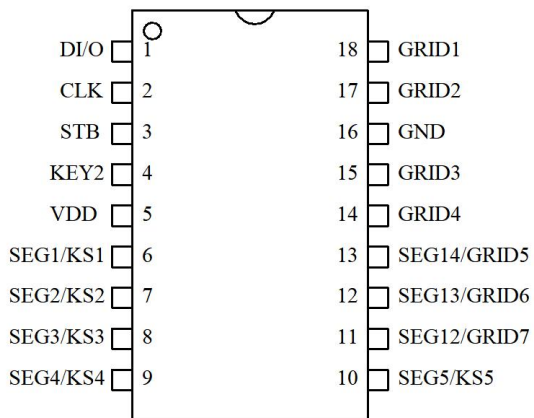
HTM1618 SOP-18
