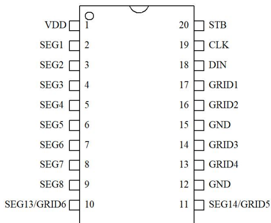
HTM1620 SOP-20
