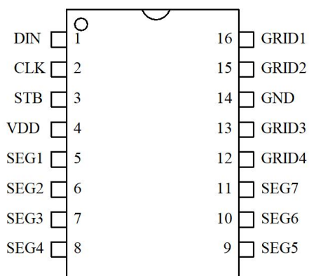
HTM1616 SOP-16
