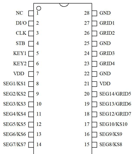
HTM1667 SOP-28
