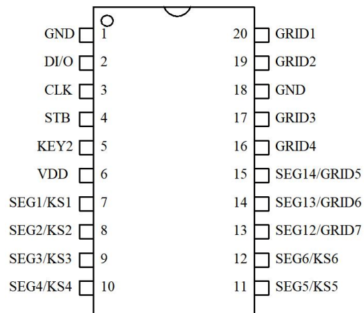
HTM1620B SOP-20
