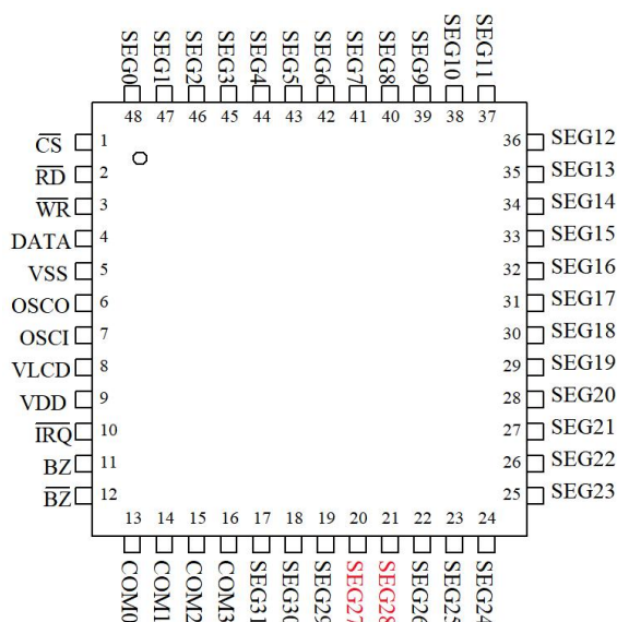
TM1621D LQFP-48
