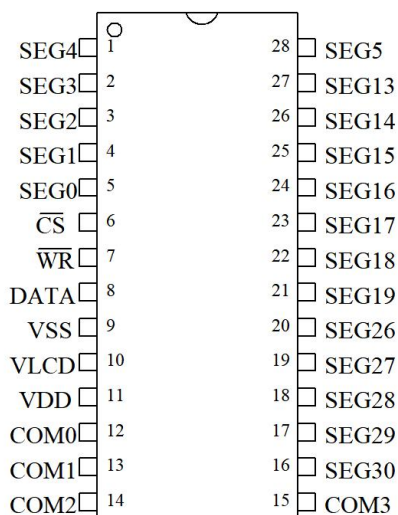
TM1621D SOP/SSOP-28
