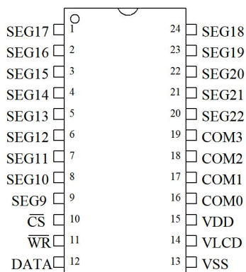
TM1621D SOP/SSOP-24
