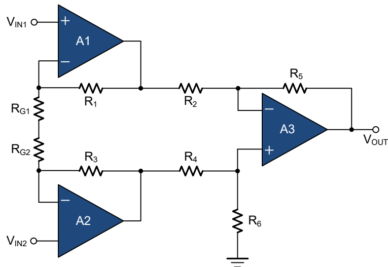
Figure10. Discrete3-Op-amp Instrumentation Amplifier
