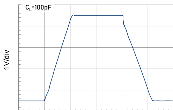
2.5μs/div Large Signal Step Response (4V Step).
