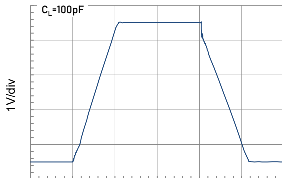
2.5μs/div Large Signal Step Response (4V Step).
