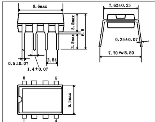
DIP 8
