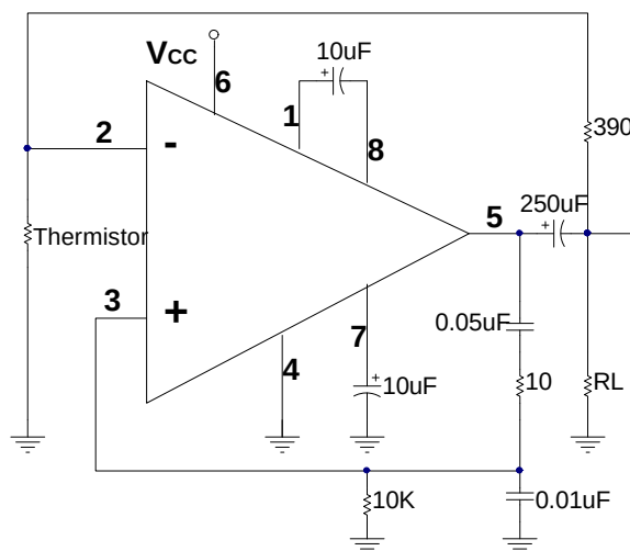
Figure 4 . Low distortion bridge oscillator
