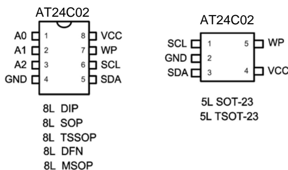
Figure 1: Package types
