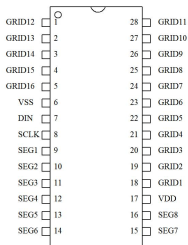
TM1640 SOP/SSOP-28
