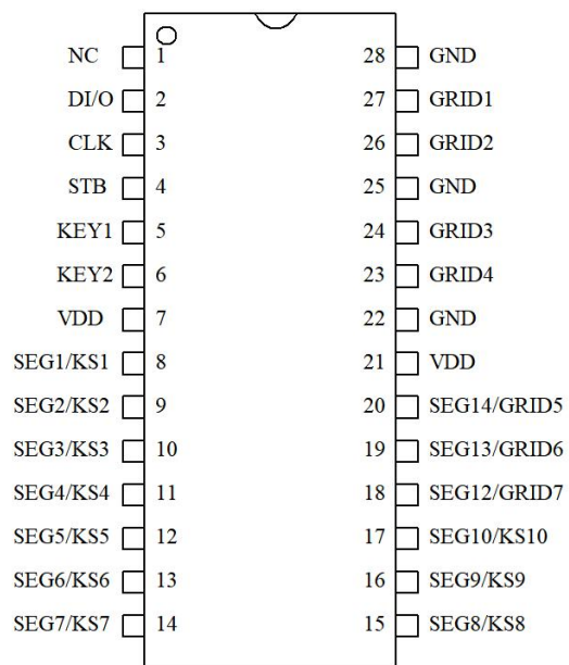
TM1628 SOP/SSOP-28
