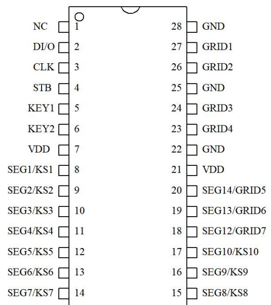
TM1667 SOP-28
