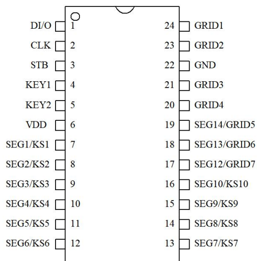
TM1668 SOP/SSOP-24
