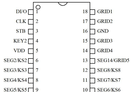
TM1630 DIP-18
