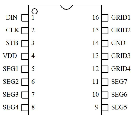
TM1616 SOP-16
