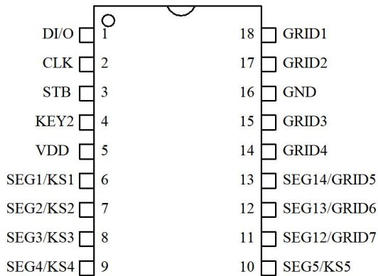
TM1618 SOP-18
