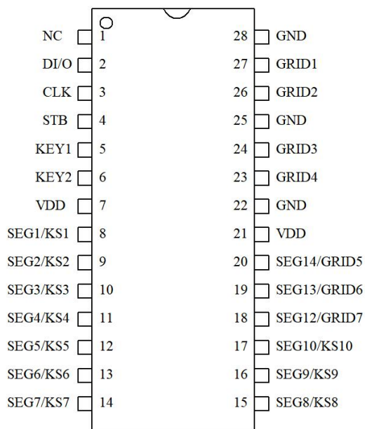
AIP1628 SOP/SSOP-28
