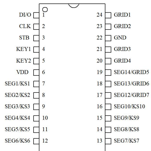
AIP1668 SOP/SSOP-24
