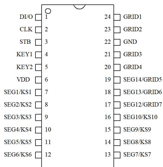
TM1668 SOP/SSOP-24
