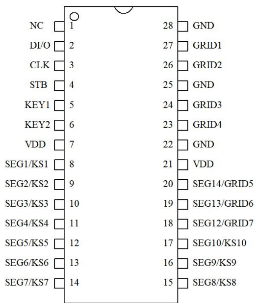
TM1628 SOP/SSOP-28
