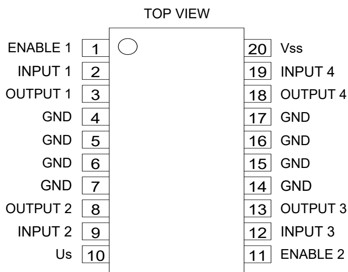
SOP-20
