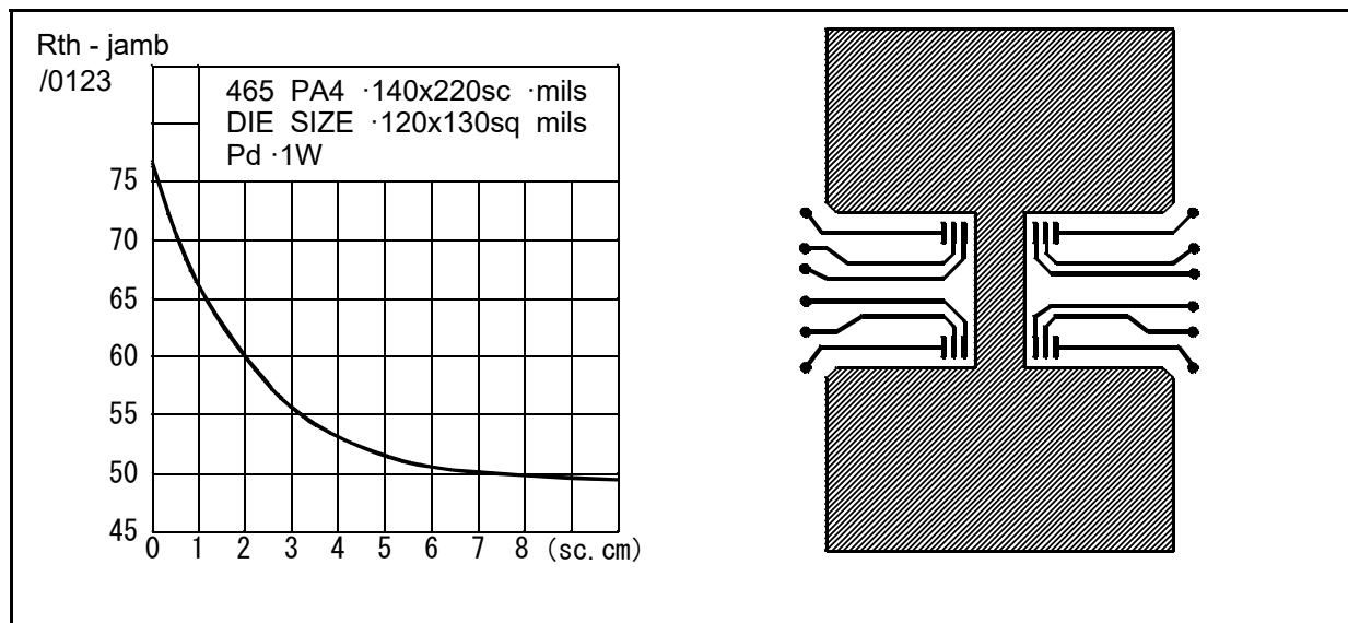
Figure 2: Junction to ambient thermal resistance vs. area on board heatsink (SOP-20 package)
