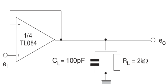
Voltage follower
