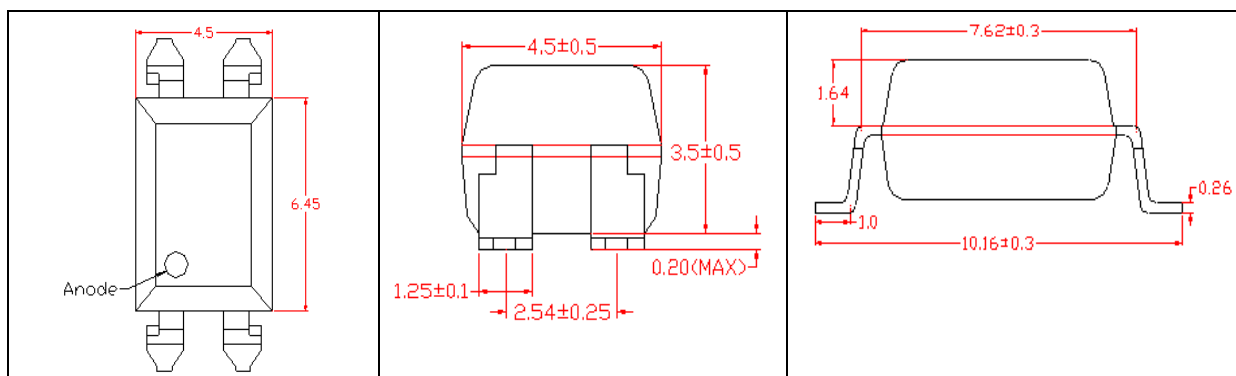
4-pin SMD(SMD-4P)
