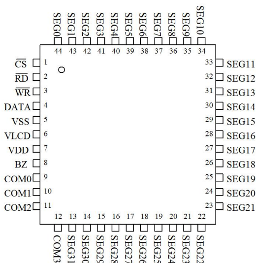
HT1621B LQFP-44
