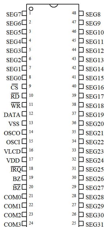
HT1621B SSOP-48
