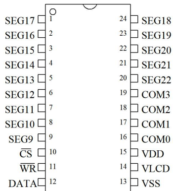
HT1621B SOP/SSOP-24
