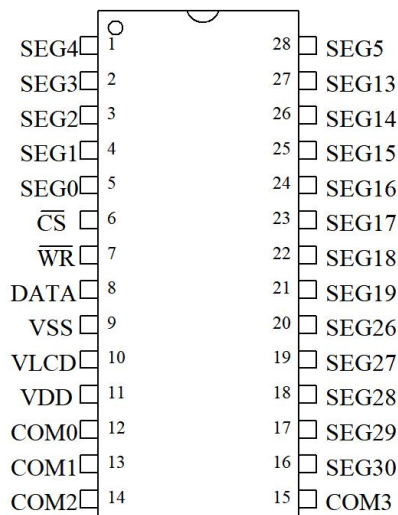
HT1621B SOP/SSOP-28
