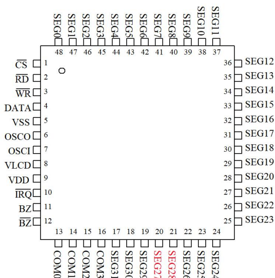
HT1621B LQFP-48
