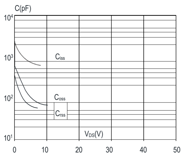
Figure 6: Capacitance Characteristics
