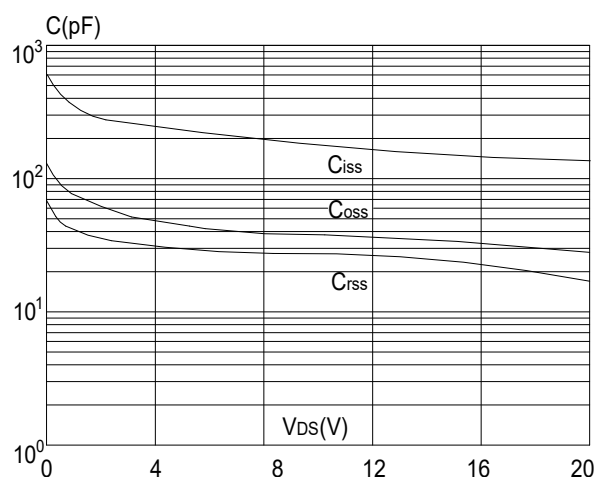
Figure 6: Capacitance Characteristics
