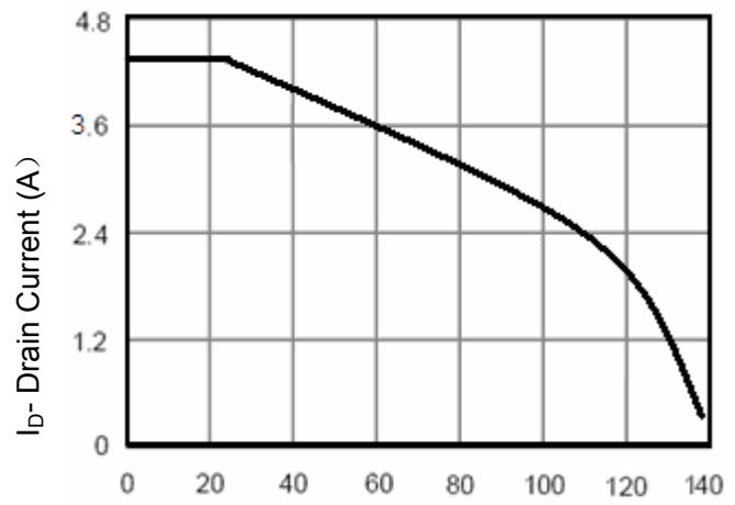
T_J -Junction Temperature( ^{\circ} C) Figure 2 Drain Current
