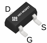
SOT-23 (TO-236AB)
