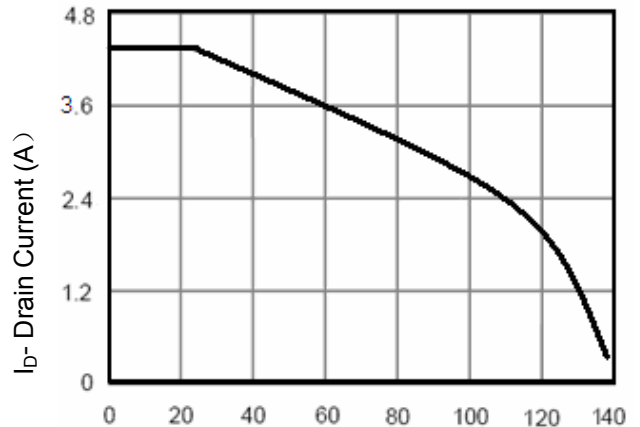
Figure 4 Drain Current
