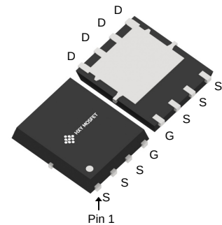
DFN5X6-8L (PQFN-8(5x6))
