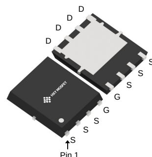
DFN5X6-8L (SO-8-FL-5.8mm)
